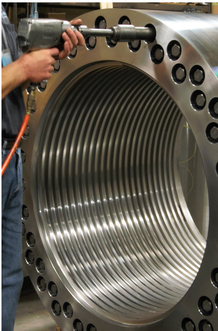
Assembling an enormous 1016 mm (40 inch) thread tensioner, used on a 50,000 ton press.
