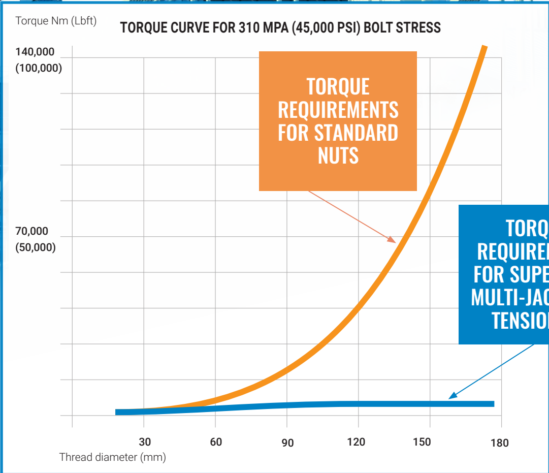
The chart shows how Superbolt tensioners remain easy to install, even on larger sizes, compared to standard hex nuts. Only hand tools are required to tighten any diameter stud/bolt.
